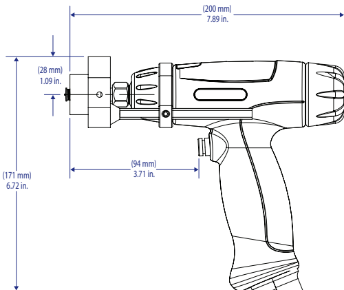
CL and GL Models with a foot and spark shield
